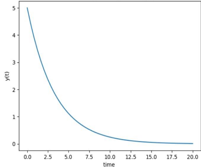
Solution of dy/dt=-ky;k=0.3,y(0)=5
